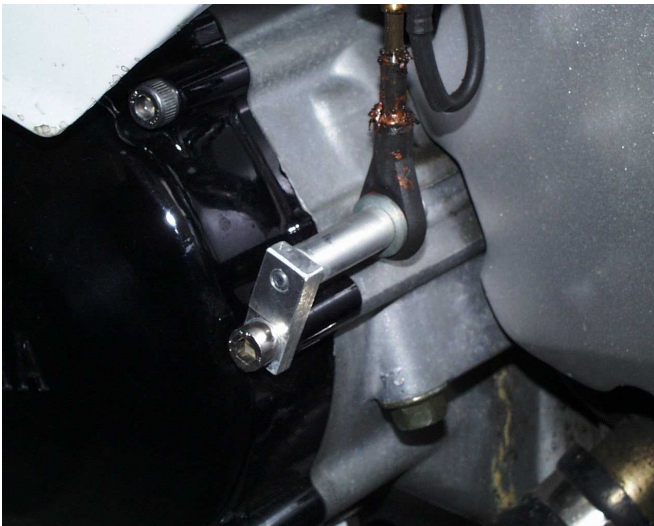
Figure 2: Lower attachment of reset sensor (rod with magnet).
