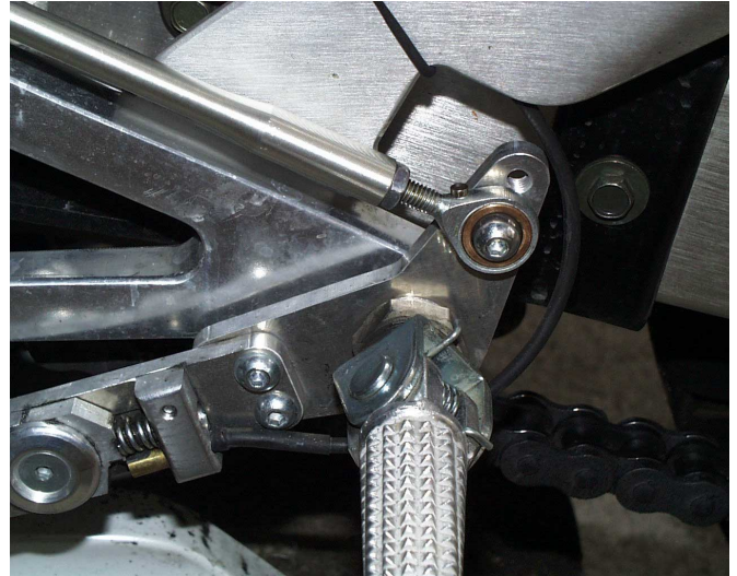
Figure 3: Recommended attachment of rod at gear-shift lever. Rod has to be mounted outside the frame.
