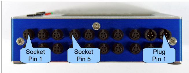
Figure 3: SICOLOG pin assignment.
